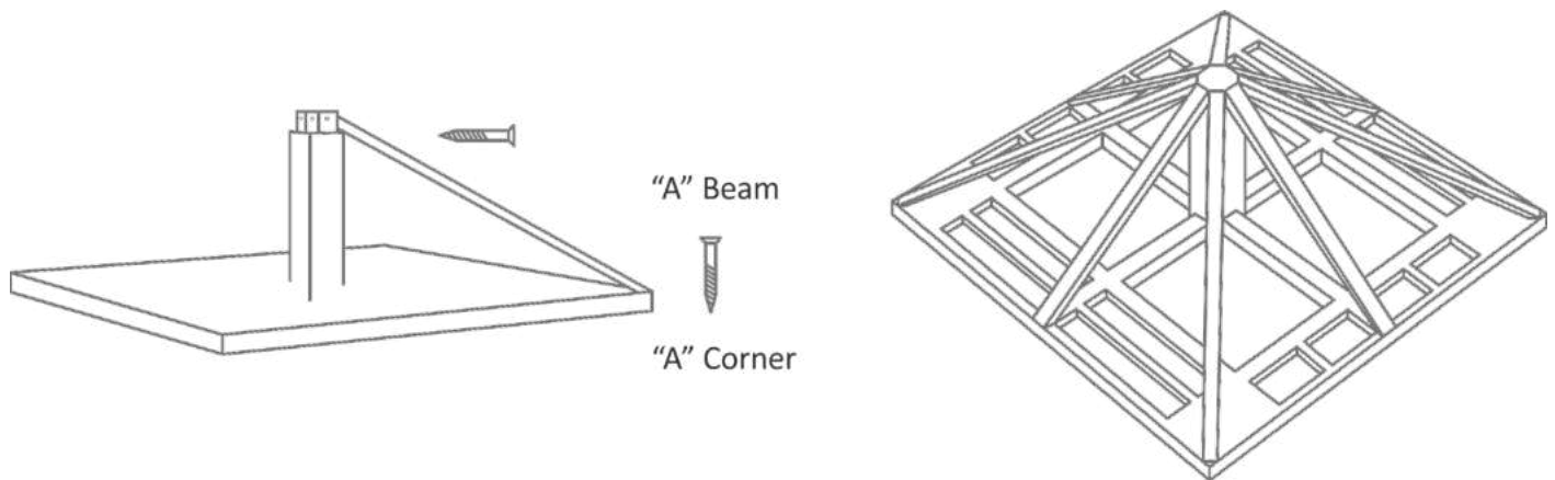
Figure D-2: Shingles Support Beams
