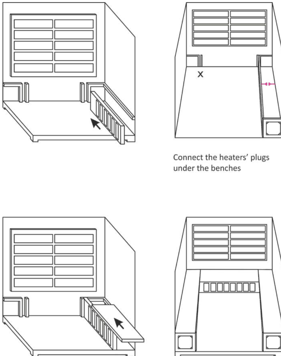
Figure C-4: Installing the Bench
